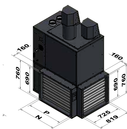
Side/Rear Dampers
