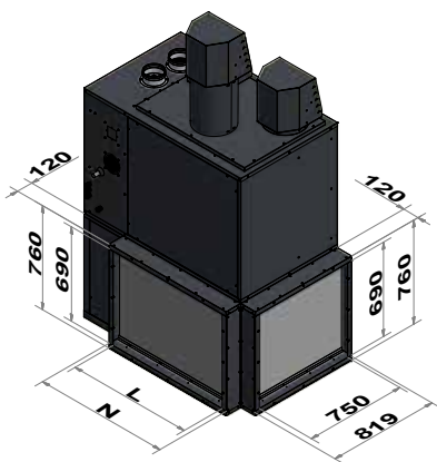
Side/Rear Filters
